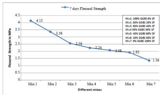
Fig.4.5 Variation in the flexural strength of GPC at 7 days of ambient curing
