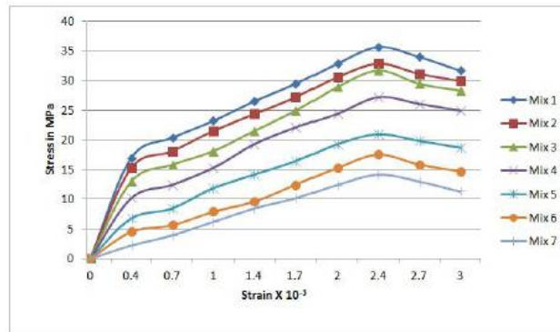
Fig.4.7 Variation in the Stress-Strain curves of GPC
