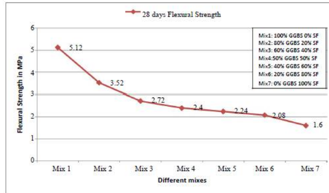
Fig.4.6 Variation in the flexural strength of GPC at 28 days of ambient curing
