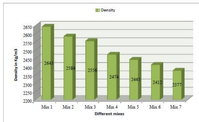
Fig.4.9 Variation in the density of GPC
