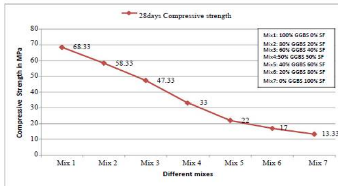
Fig.4.2 Variation in the compressive strength of GPC at 28 days of ambient curing
