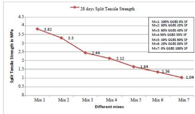
Fig.4.4 Variation in the split tensile strength of GPC at 28 days of ambient curing
